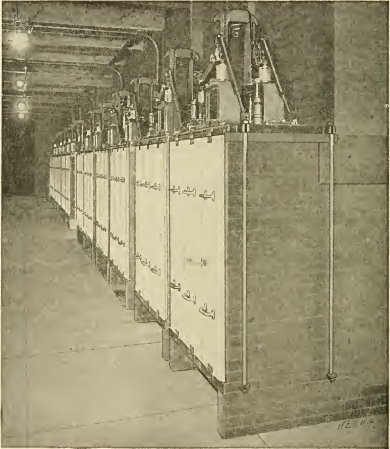
Fig. 161. Installation of Westinghouse Type C Electrically-Operated, Distant-Control Circuit Breakers
